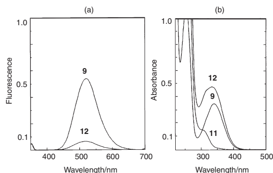
Figure 1. (a) Fluorescence emission spectra of 9 and 12 in acetonitrile ( 0.2 \times 10^{-4} M) at room temperature. (b) UV-vis absorption spectra of 9 , 11 , and 12 in acetonitrile ( 1.0 \times 10^{-4} M) at room temperature.
