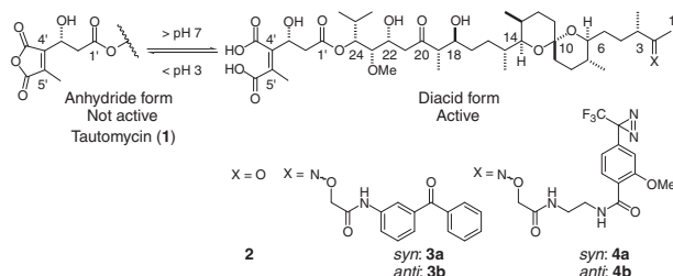
Scheme 1. Tautomycin and photoaffinity probes.
