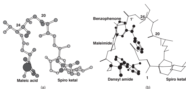
Figure 2. Proposed 3-D structures of 2 and 12 ; (a) One of the stable conformations of 2 ; (b) One of the energy-minimized conformations of 12 on the basis of 2 .
