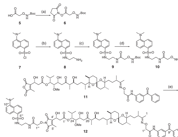
Scheme 2. Synthesis of fluorescent photoaffinity probe: (a) N -hydroxysuccinimide, EDC·HCl, DMF, rt, 36 h, 78%; (b) ethylenediamine, Et 3 N, CH 2 Cl 2 , rt, quant.; (c) 6 , Et 3 N, DMF, rt, 1 h, 68%; (d) TFA/CH 2 Cl 2 (1:1), 0 °C, 1 h, 87%; (e) 10 , 70% DMA/H 2 O, pH 4, rt, 16 h, then purification by HPLC, 83%.
