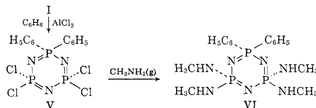
CHART III ARYLATION AND AMINOLYSIS DERIVATIVES OF BIS-N-METHYLAMINOTETRACHLOROTRIPHOSPHONITRILE
