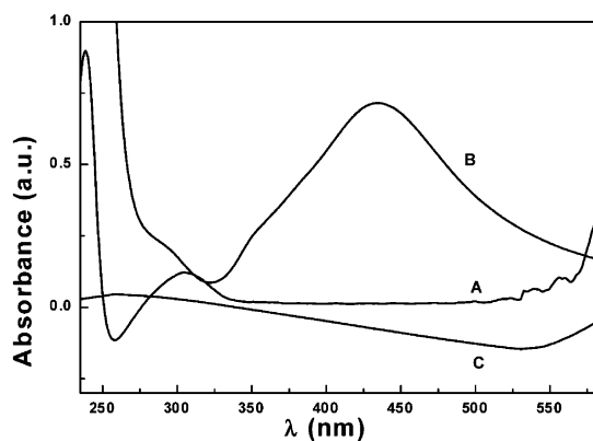
Figure 4. UV-visible absorption spectra recorded after 2 min of silver nanocluster formation under various conditions in (A) aq 1,4-dioxan, (B) \text{AgNO}_3 and aq \text{NH}_3 , and (C) \text{AgOCOPh} and 2-hexanone-1-diazo-6-phenyl.
