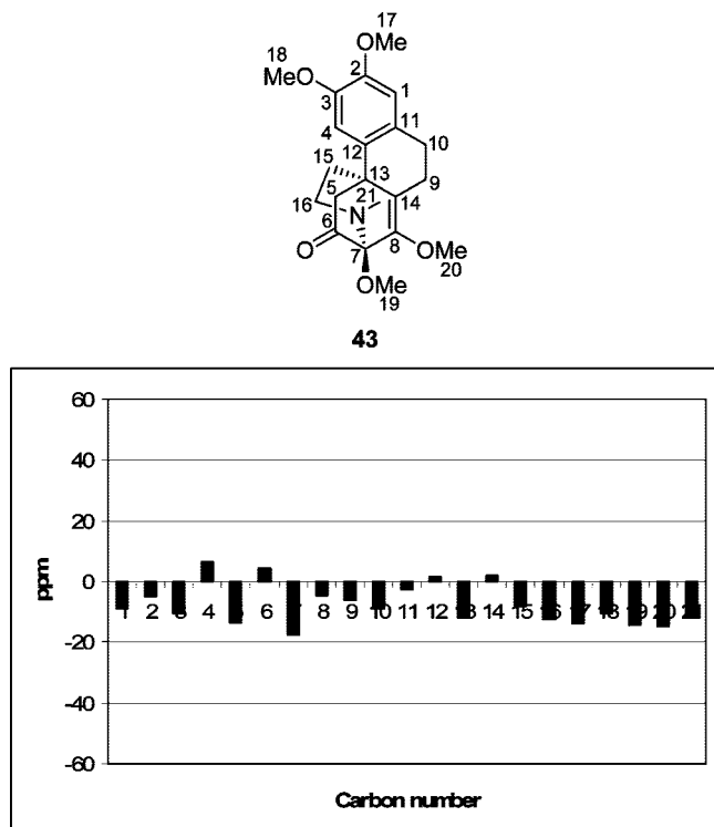
FIGURE 9. Difference between calculated and experimental ^{13}\text{C} NMR shifts for isorunanine ( 43 ) in benzene. The average |\Delta\delta| was 9.1 ppm, and the maximum was 17.4 ppm.
