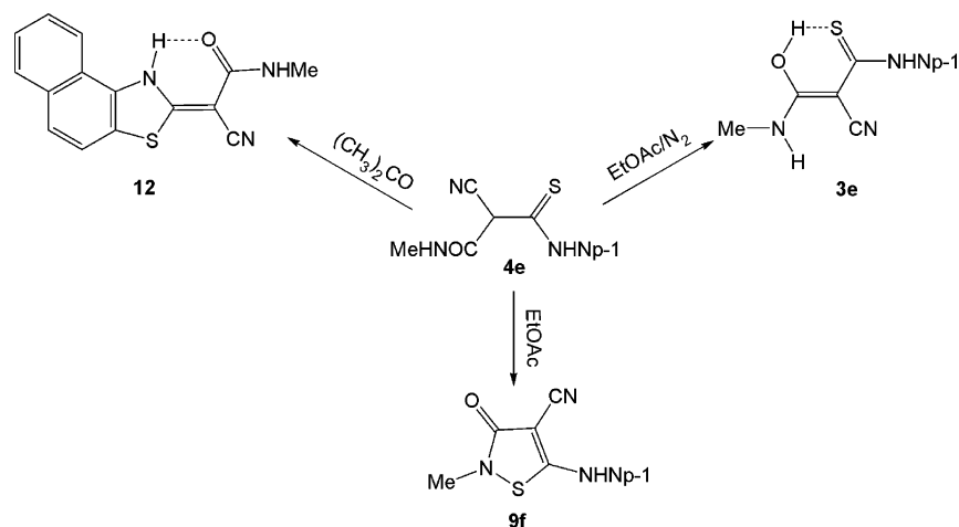
SCHEME 8. The Various Products Formed from Formal 4e
