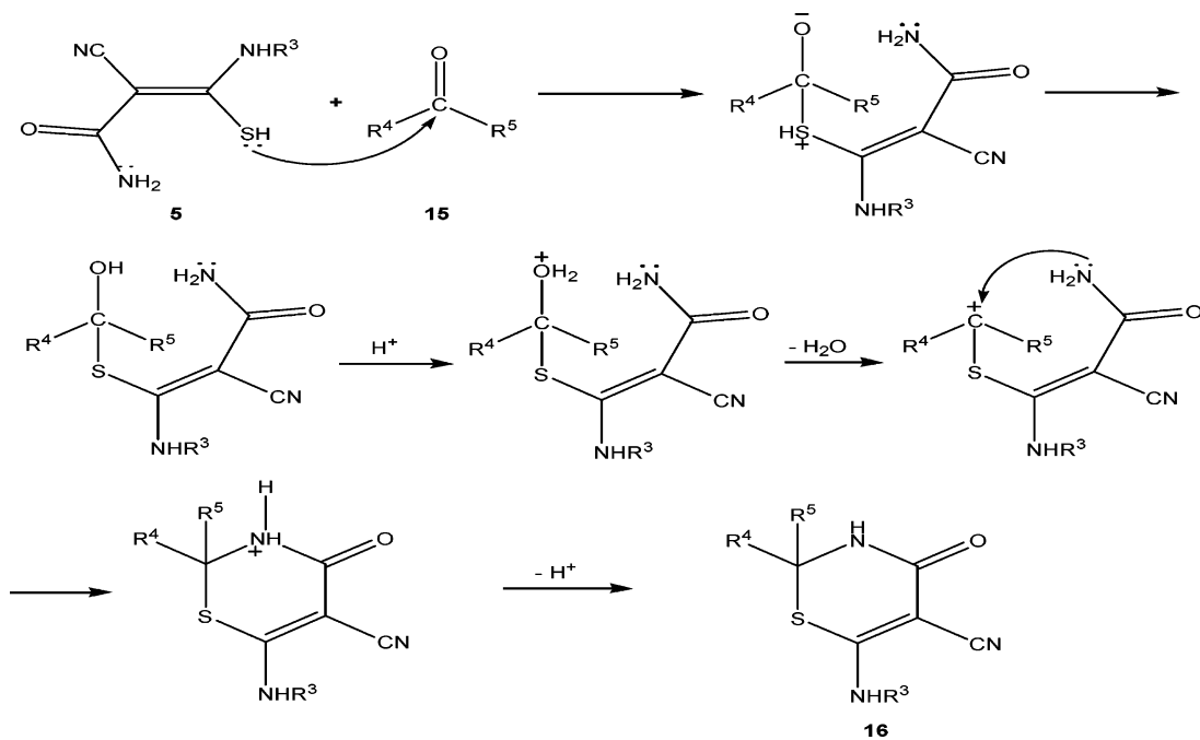
SCHEME 2. Suggested Mechanism for a Formation of 20
