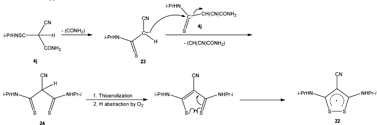
SCHEME 4. Suggested Mechanism for Formation of 22
