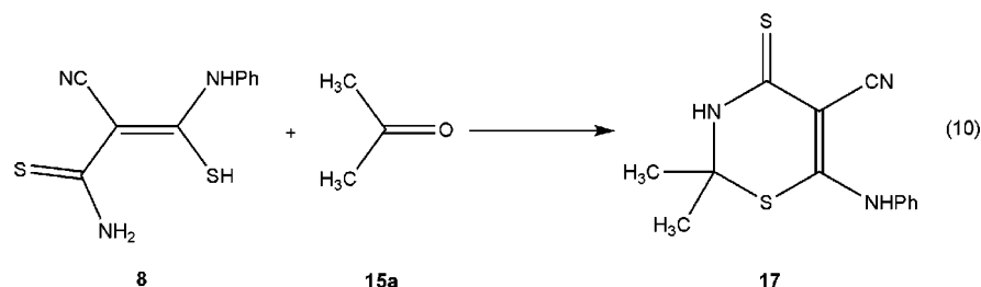
SCHEME 2. Suggested Mechanism for a Formation of 20
