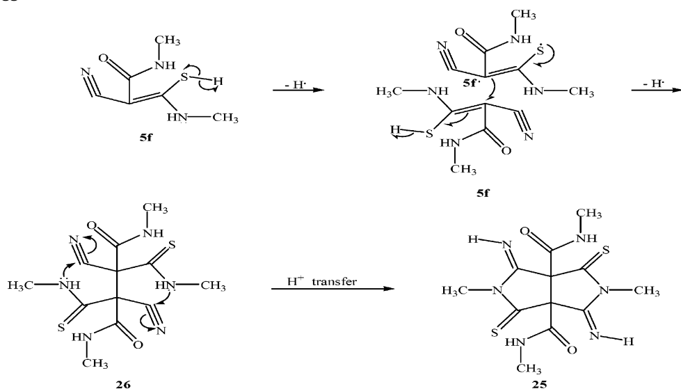
SCHEME 5. Suggested Mechanism for a Formation of 25
