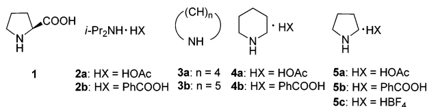
Figure 1. Organocatalysts 1–5 .
