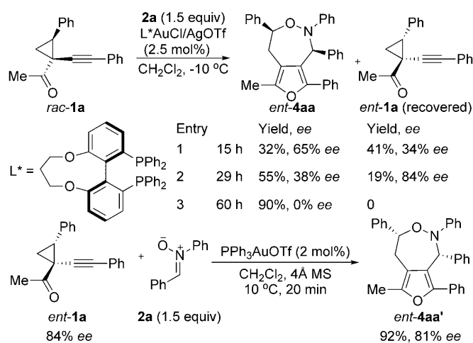
Scheme 3. Kinetic resolution of rac - 1a and transformation of the recovered ent - 1a ; L* = ( R )-C 3 -TunePhos.
