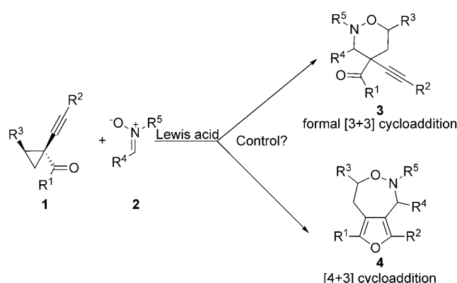
Scheme 1. Proposed reaction pattern for 1-(1-alkynyl)cyclopropyl ketones with nitrones.
