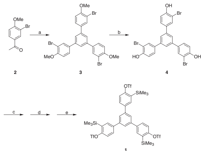
Scheme 1. (a) \text{TiF}_2\text{O} , toluene, reflux, 55%; (b) \text{HBr} , \text{AcOH} , 75^\circ\text{C} , 67%; (c) \text{HMDS} , 70^\circ\text{C} ; (d) \text{Me}_3\text{SiCl} , \text{Na} , toluene, reflux; (e) (i) n\text{-BuLi} , \text{Et}_2\text{O} , 0^\circ\text{C} to rt; (ii) \text{TiF}_2\text{O} , 0^\circ\text{C} to rt, 27% (from 4 ).
