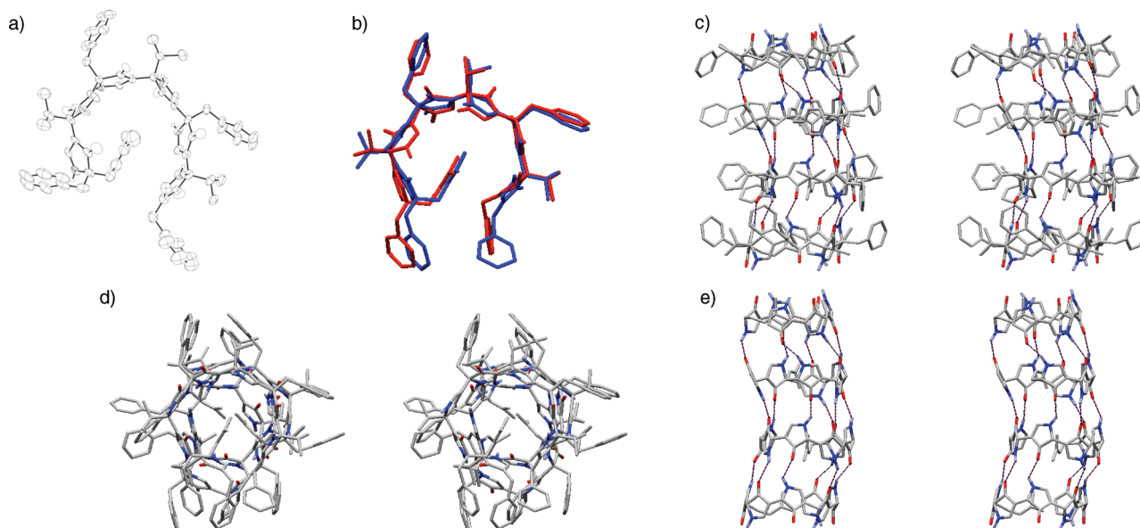
Figure 3. (a) ORTEP diagram of the D,L-mixed hexapyrrolinone (-)-4 . (b) Overlay of the crystal structure (blue) and the solution structure (red) of (-)-4 . (c) and (d) Stereoviews illustrating the nanotube-like assembly of (-)-4 in the crystal packing diagram, side view and top view, respectively, with intermolecular hydrogen bonding illustrated. (e) Stereoview with side-chains removed to highlight the nanotube-like assembly.
