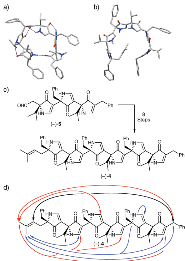
Figure 2. (a) Computational model of (-)-4 in \text{CHCl}_3 arising from a 10 000-step Monte Carlo conformational search. (b) The solution structure of the alternating D,L-hexapyrrolinone (-)-4 . (c) Synthesis of hexapyrrolinone (-)-4 . (d) Ten critical long-range NOEs, color coded by their interactions with the prenyl side chain.
