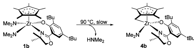
Scheme 7. Formation of “Tuck-In” Complex 4b
