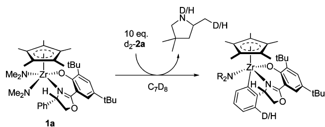
Scheme 6. Partial Deuteration of Catalyst during Reaction with N-Deuterated Substrate
