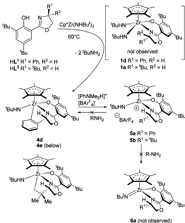
Scheme 5. Stoichiometric Reactions To Probe Activation and Deactivation Pathways
