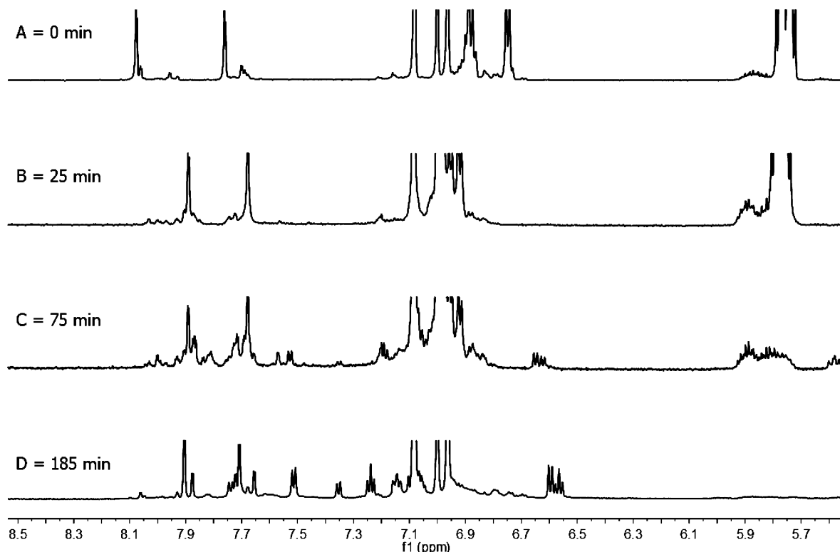
Figure 8. (A) Initial ^1\text{H} NMR spectrum ( \delta 6.5–8.5 ppm) of 1a and substrate 3a in toluene- d_8 at ambient temperature. Minor resonances correspond to the activated catalyst, where one or both \text{NMe}_2 groups have been replaced by substrate. (B) t = 25 min, showing activated catalyst but no CH-activated species. (C) t = 75 min, showing activated catalyst and a small amount of CH-activated species at a low [substrate]. (D) t = 185 min, showing several CH-activated species but no coordinated or free substrate.
