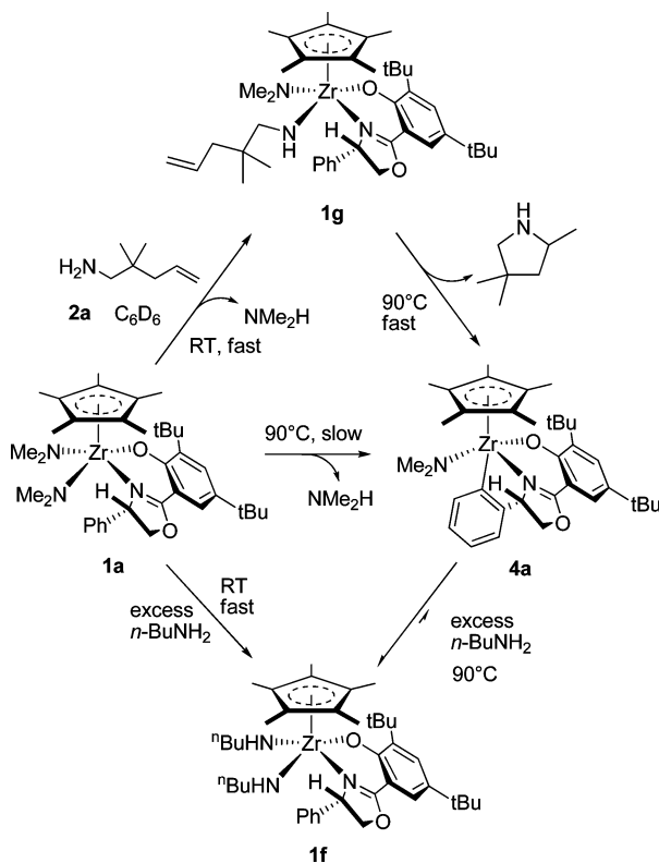
Scheme 5. Stoichiometric Reactions To Probe Activation and Deactivation Pathways
