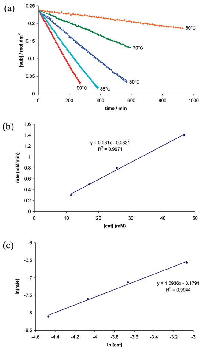
Figure 1. Kinetic plots of hydroamination/cyclization of 2a using precatalyst 1a in toluene- d 8 : (a) zero-order plots of [substrate] versus time, 60–90 °C; (b) determination of order with respect to catalyst at 90 °C; (c) Van't Hoff plot for 90 °C data using the precatalyst. The lines are least-squares fits to the data points.
