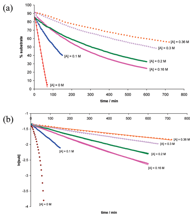
Figure 6. (a) Kinetic plots of [substrate] versus time for cyclohydroamination of 3a using precatalyst 1a in toluene- d_8 at 90 °C as a function of concentration of added n -hexylamine ( A ). (b) First-order plots of the same data. [cat.] = 0.025 M in all cases. The lines are least-squares fits to the data points.
