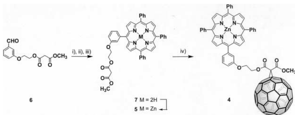
Scheme 1. Synthesis of the mono-linked 4 : i) benzaldehyde, pyrrole, \text{Ph}_4\text{PCl} , \text{BF}_3 \cdot \text{Et}_2\text{O} , \text{CH}_2\text{Cl}_2 , RT; ii) p -chloranil, reflux, (silicagel, \text{CH}_2\text{Cl}_2/\text{EtOAc} (20:1)); iii) \text{Zn}(\text{OAc})_2 \cdot 2\text{H}_2\text{O} , THF, reflux; iv) \text{C}_{60} , DBU, toluene.
