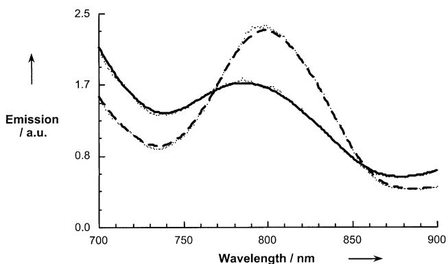
Figure 4. Charge transfer emission of ZnP–C 60 ( 4 : solid line) and ( 2 : dashed line) in toluene at 77 K ( \sim 1.0 \times 10^{-5} \text{ M} ); excitation wavelength 560 nm.
