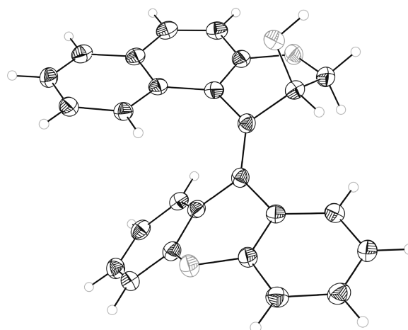
Figure 1. Molecular structure of 2c in the crystal.
