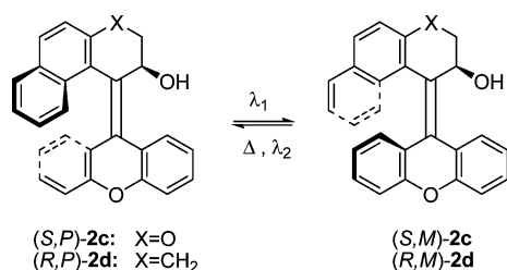
Scheme 9. Light-Induced Interchange Between the Respective P - and M -Forms of the Aromatic Optical Switches 2c,d
