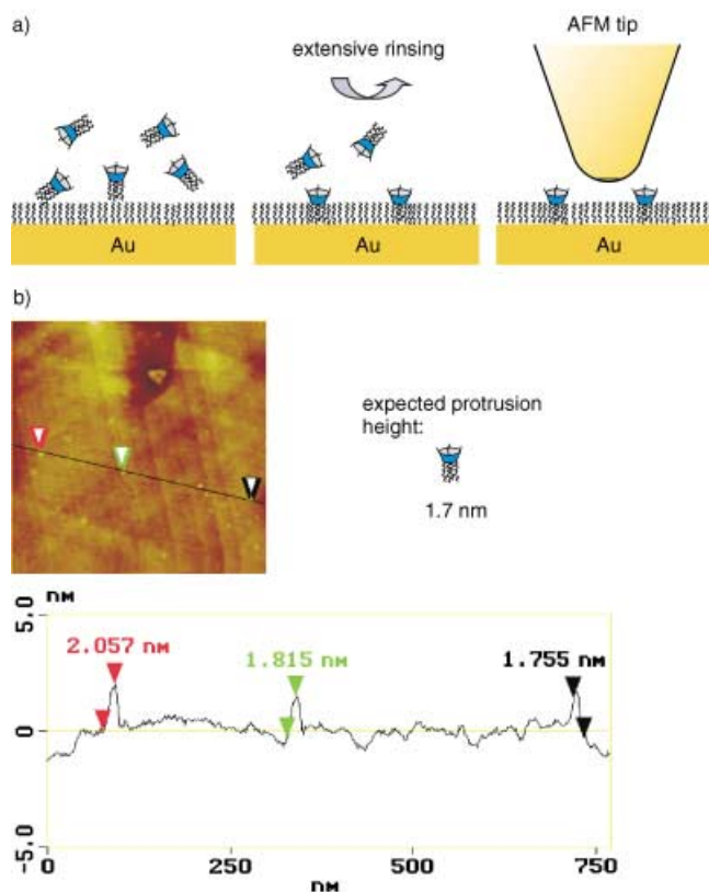
Figure 3. a) Schematic representation of cavitand 6 insertion and AFM analysis on MU SAM; b) TM-AFM image and section analysis of a MU SAM with inserted phenylpyridine functionalized thioether-footed cavitand 6 .
