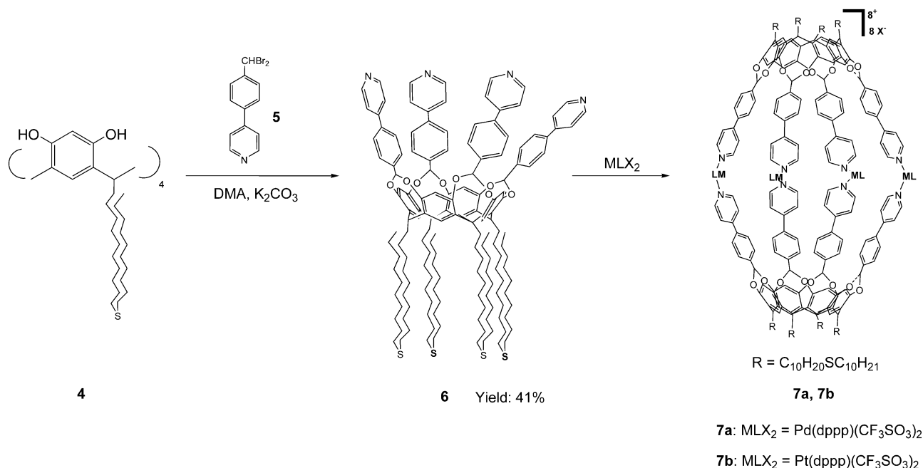
Scheme 2. Synthesis of the cavitand ligand 6 , and self-assembly of nanosize coordination cages 7a and 7b .
