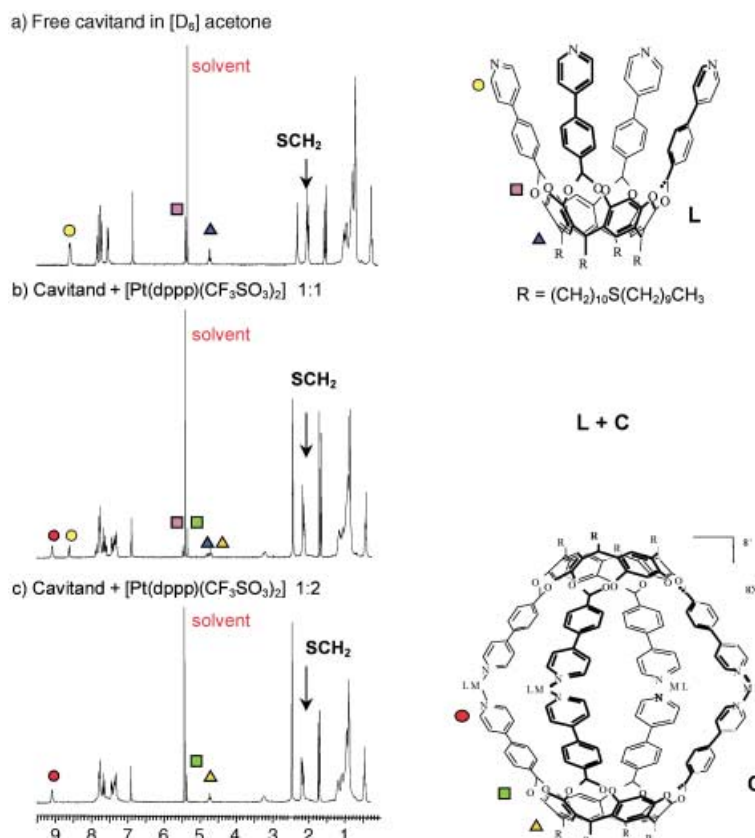
Figure 1. Self-assembly of cage 7b in solution monitored by ^1\text{H} NMR spectroscopy.
