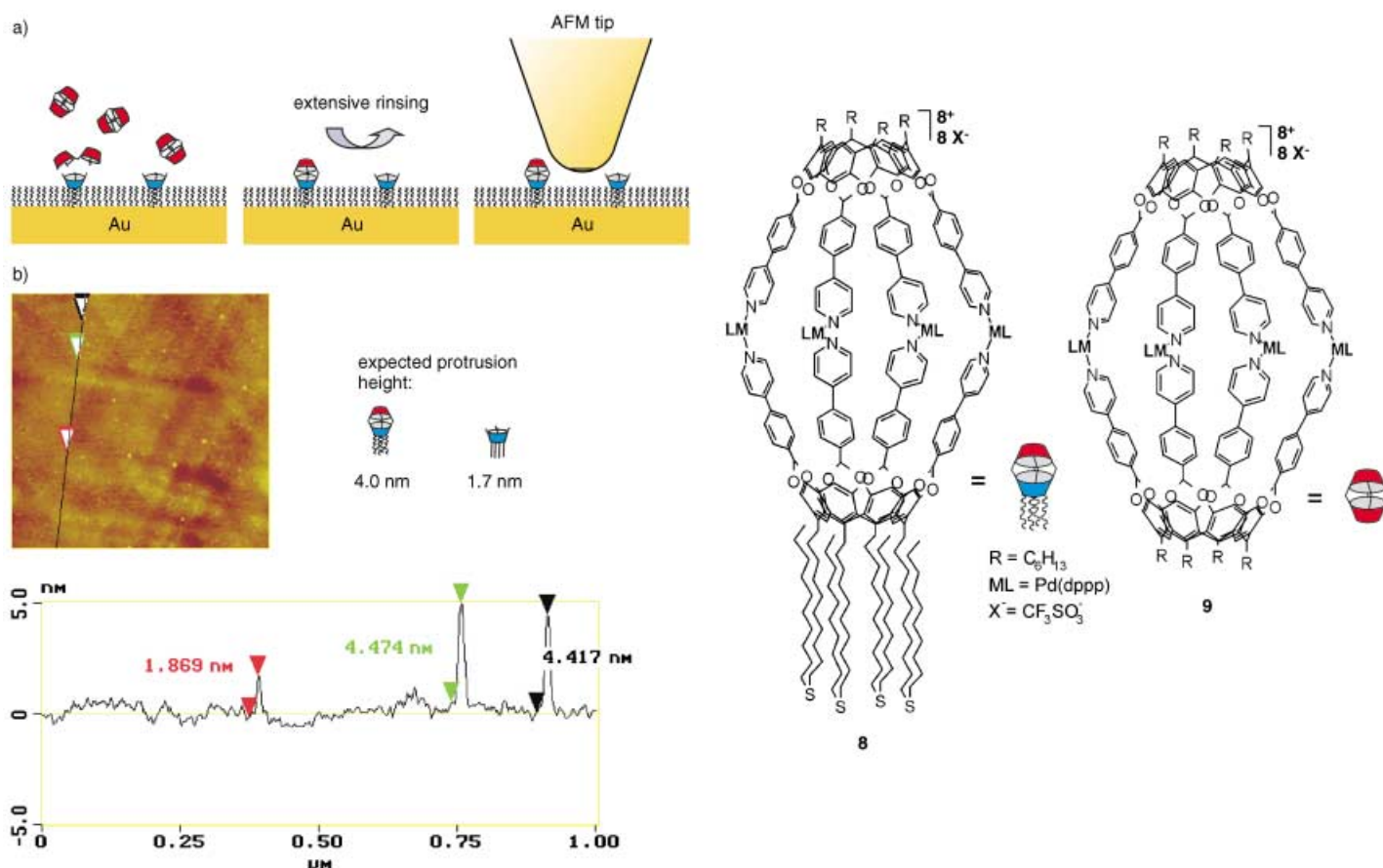
Figure 4. a) Schematic representation of the surface assembly of heterocages 8 from surface bound cavitands with cages in solution; b) TM-AFM image and section analysis of a MU SAM with heterocages 8 (green and black) and cavitands (red).
