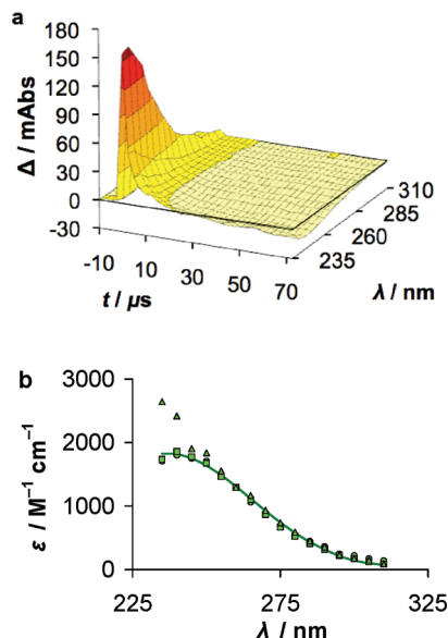
Figure 5. Spectral changes upon photolysis (266 nm, 100 mJ/pulse) of 1.1 mM (Me 4 N)ONOO − at pH 4.8 and 25 °C, prepared from equal volumes of 2.2 mM (Me 4 N)ONOO in 10 mM KOH and a 0.1 M pivalate buffer. (a) Spectrum as a function of time after the pulse, showing apparent second-order decay via recombination of HO 2 •/O 2 • − with NO•, ca. 125 μM yield of HO 2 •/O 2 • − . In contrast to photolysis at 355 nm (Figure 3a), the absorbance of the reaction mixture decays to a level lower than the initial level. (b) Spectral data, corrected for the bleaching of ONOOH, recorded at 0.07 μs (green circles) and 5 μs (green triangles) after photolysis of ONOOH at pH 4.8 and calculated spectrum of HO 2 •/O 2 • − at pH 4.8 (green line), as in Figure 3b. Data points are derived from the data in a. In contrast to photolysis at 355 nm (Figure 3b), a systematic deviation from a model for exclusive formation of NO• and HO 2 • (reaction 5) is observed at λ > 300 nm for 0.07 μs time points (circles) and at λ < 250 nm for 5 μs points (triangles).
