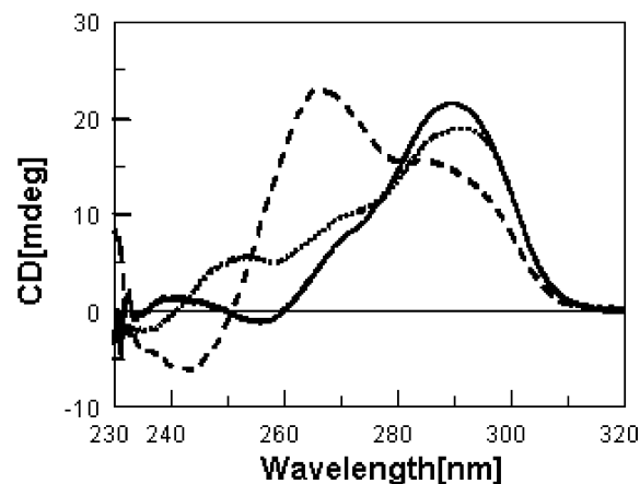
Figure 4. CD spectra of 4 \mu M 4GGG incubated for 24 h alone (solid line) and in the presence of 26 \mu M 5 at 25 °C (dotted line) or 40 °C (dashed line) in \text{Li}_3\text{PO}_4 10 mM, KCl 50 mM, pH 7.4.
