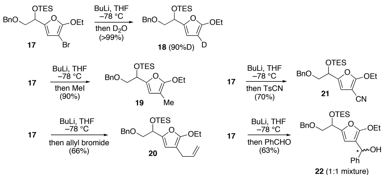
Scheme 4. Conversion of 3-bromofuran 17 to various 3-substituted furans ( 18–22 ).
