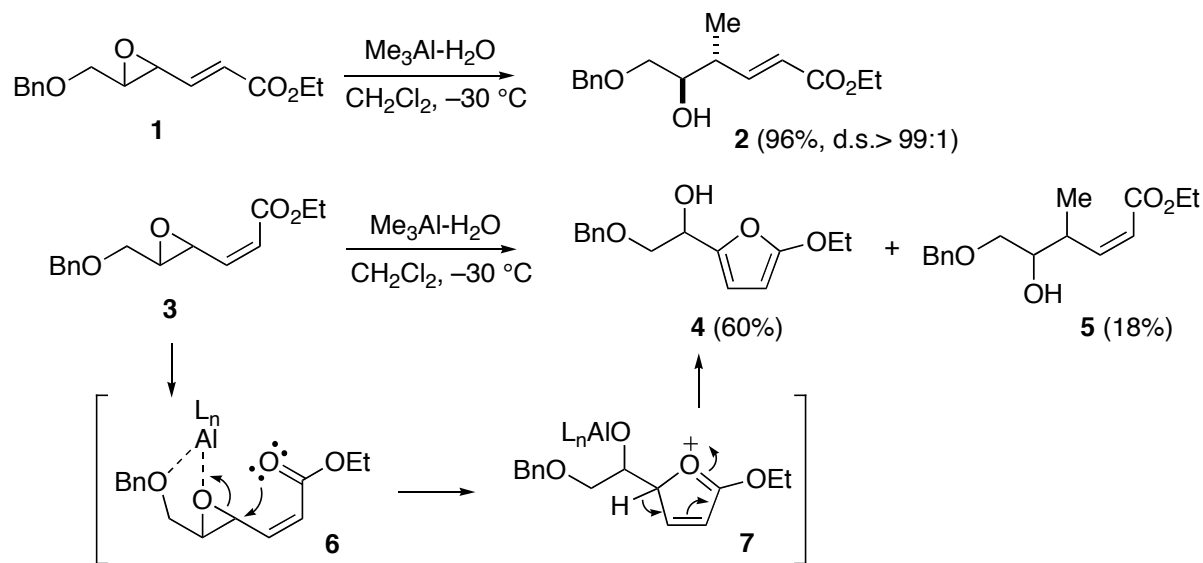
Scheme 1. The reactions of \gamma,\delta -epoxy-( E )-acrylate 1 and ( Z )-acrylate 3 with \text{Me}_3\text{Al-H}_2\text{O} .
