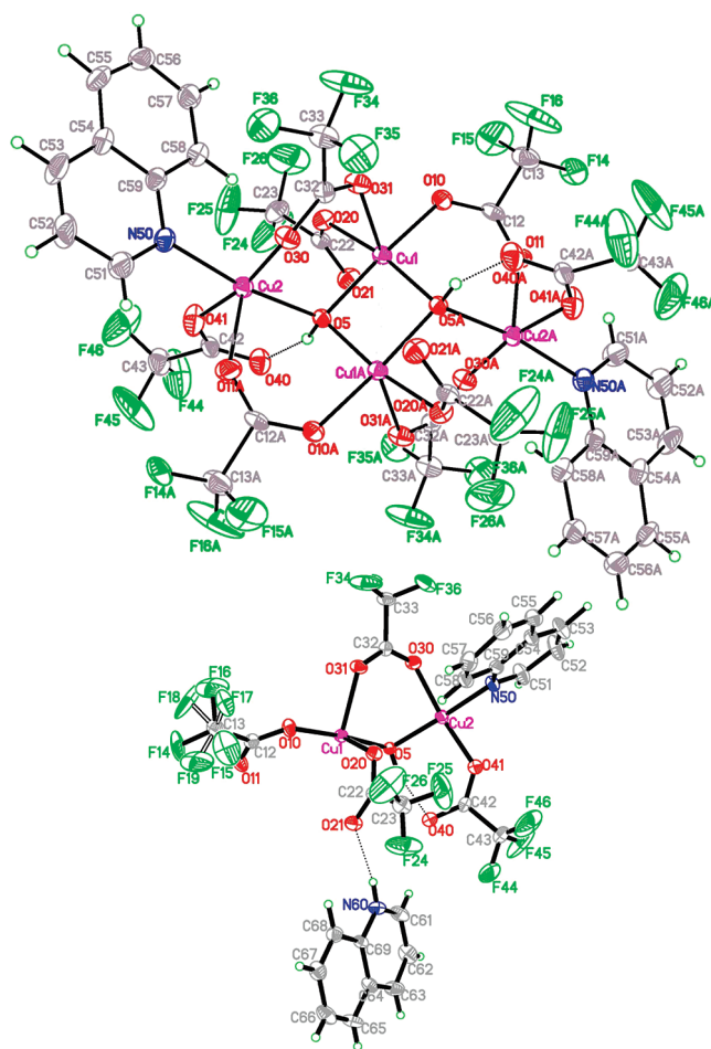
Figure 2. (Top) Structure of the tetranuclear anion [\text{Cu}_2\text{OH}(\text{CF}_3\text{COO})_4(\text{quin})]^{2-} in 2a . (Bottom) One-half of the tetranuclear anion and the noncoordinated \text{quinH}^+ cation forming hydrogen bonds \text{N60-H60}\cdots\text{O21} (1.95 Å) and \text{N60-H60}\cdots\text{F24} (2.82 Å) to the anion.
