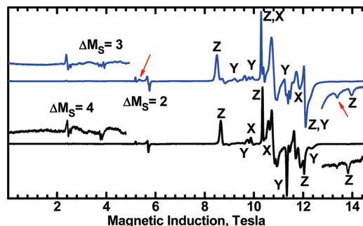
Figure 7. EPR spectra of 3 (bottom) and of 4 (top) at 15 K and 324 GHz. The molecular orientations for the resonance lines are marked by X, Y and Z. The distance between the outer Z lines is 5.48 T in 4 and 5.18 T in 3 . Arrows indicate signals due to frozen oxygen ( S = 1 , g_{\text{iso}} = 2 , D = 3.57 \text{ cm}^{-1} ) that is frequently observed below T = 30 \text{ K} . 48
