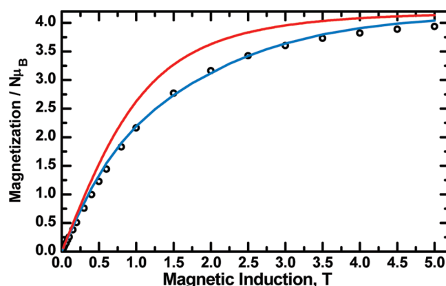
Figure 4. Magnetization of 4 , in multiples of N\mu_B , measured at 1.8 K (black circles). The theoretical saturation value equals gS . Blue line: magnetization calculated as \chi B/N\mu_B with inclusion of the zero-field splitting using \chi from eq 4. Red line: calculated from the Brillouin function including only the Zeeman term: M = -g \sum_{m=-2}^2 m \exp(-g\mu_B B m/kT) / \sum_{m=-2}^2 \exp(-g\mu_B B m/kT) . g = 2.09 was used in both calculations.
