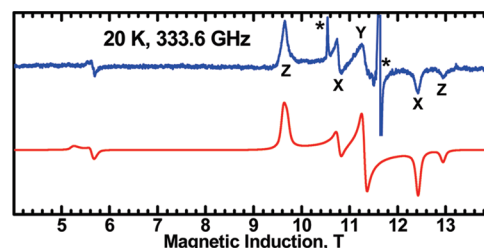
Figure 11. Blue: EPR spectrum of 3a . Asterisks indicate resonances due to a monomeric copper species. Sharp “perpendicular” part of the monomer signal is cut off to make the triplet spectrum better visible. Red: Spin-triplet spectrum simulated with g_x = 2.049 , g_y = 2.263 , g_z = 2.112 , D = -1.636 \text{ cm}^{-1} , E = -0.0187 \text{ cm}^{-1} .
