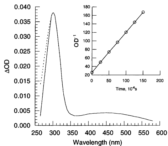
Figure 1. Differential absorption spectrum of PhSO^\bullet radical after excitation of 8 (X = H, 6.2 \times 10^{-5} M) in air-saturated cyclohexane (solid line). Absorption spectrum of PhSO^\bullet corrected for ground state bleaching of sulfoxide (dashed line). Insert: Second order plot of the decay kinetics at 300 nm in the same solution.
