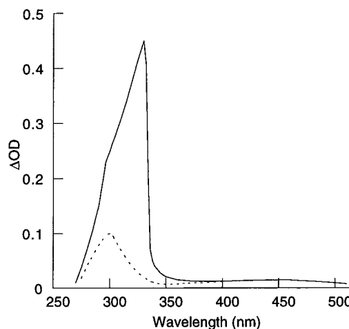
Figure 3. Absorption spectrum of transients after excitation of 4 ( 6.5 \times 10^{-5} \text{ M}^{-1} \text{ s}^{-1} ). The solid line is immediately after the laser pulse in Ar-flushed acetonitrile, and the dashed line is for an \text{O}_2 -saturated solution, taken 100 ns after the pulse.
