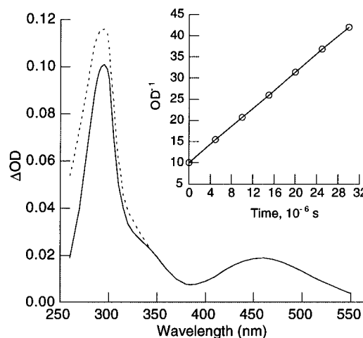
Figure 4. Differential absorption spectrum of \text{PhS}^{\bullet} after excitation of \text{PhSSPh} ( 5.5 \times 10^{-5} \text{ M} ) in air-saturated acetonitrile (solid line). Absorption spectrum of \text{PhS}^{\bullet} corrected for ground state bleaching of sulfide. Insert: Second order plot of the decay kinetics at 295 nm.
