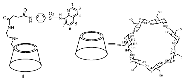
Scheme 1. HQAS-modified \beta -CD.
