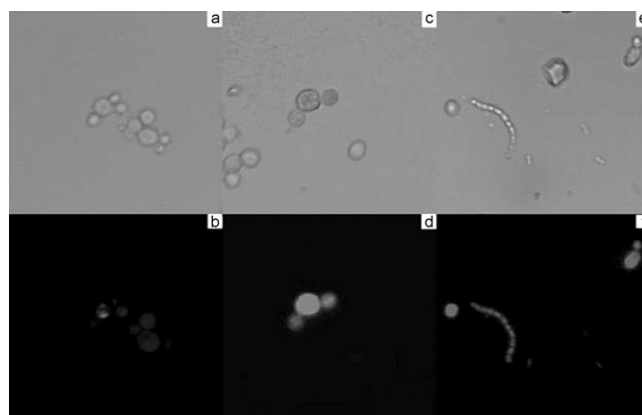
Figure 5. a) Optical and b) fluorescence microscopic images of yeast cells in the presence of 1 (50 \mu\text{M} ), c) optical and d) fluorescence microscopic images of yeast cells in the presence of 1 (50 \mu\text{M} ) and \text{ZnSO}_4 (50 \mu\text{M} ), e) optical and f) fluorescence microscopic images of killed yeast cells in the presence of 1 (50 \mu\text{M} ) and \text{ZnSO}_4 (50 \mu\text{M} ).
