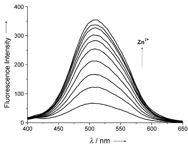
Figure 1. Emission spectra (excitation at 360 nm) of 1 ( [\mathbf{1}] = 20 \mu\text{M} ) with the addition of \text{Zn}^{2+} ( [\text{Zn}^{2+}] = 0, 2, 4, 6, 8, 10, 12, 14, 16, 18 \mu\text{M} ) in buffer solution (pH 7.2) at 25 °C.
