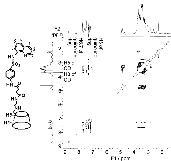
Figure 3. ROESY spectrum of 1 (2 mM) in \text{D}_2\text{O} at 25 °C.
