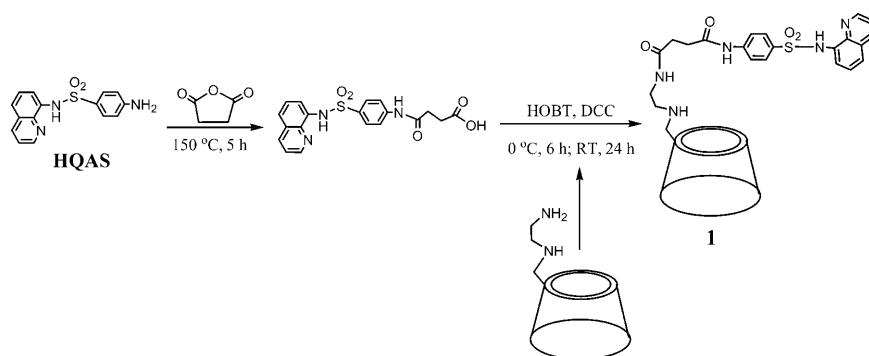
Scheme 2. The synthesis method of 1 .
