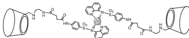
Scheme 3. Possible structure of \text{Zn}\cdot\mathbf{1}_2 .
