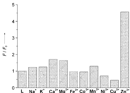
Figure 2. Relative fluorescence intensities of 1 ( [\mathbf{1}] = 20 \mu\text{M} ) in the presence of various cations ( [\text{Na}^+] = [\text{K}^+] = [\text{Ca}^{2+}] = [\text{Mg}^{2+}] = 5 \text{ mM} , [\text{Zn}^{2+}] = [\text{Cu}^{2+}] = [\text{Ni}^{2+}] = [\text{Co}^{2+}] = [\text{Fe}^{2+}] = [\text{Mn}^{2+}] = 10 \mu\text{M} ). These data were measured at pH 7.2 ( \lambda_{\text{ex}} = 360 \text{ nm} , \lambda_{\text{em}} = 506 \text{ nm} ).
