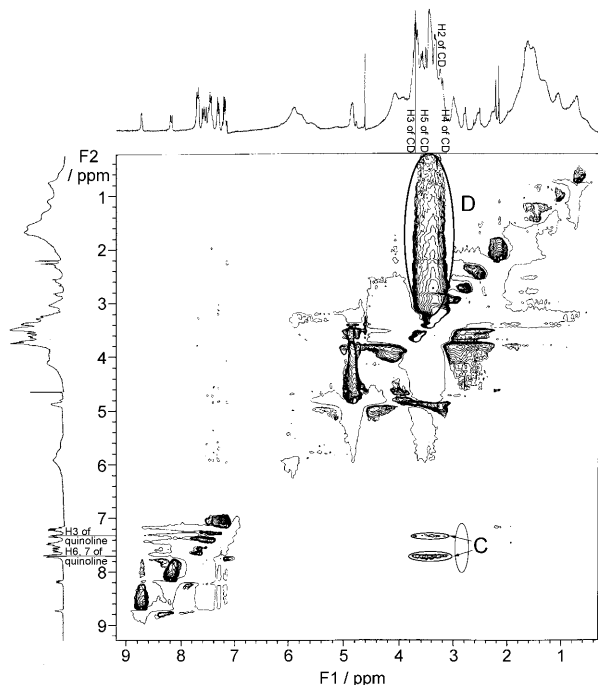
Figure 4. ROESY spectrum of 1 (2 mM) in the presence of liposome at 25 °C.
