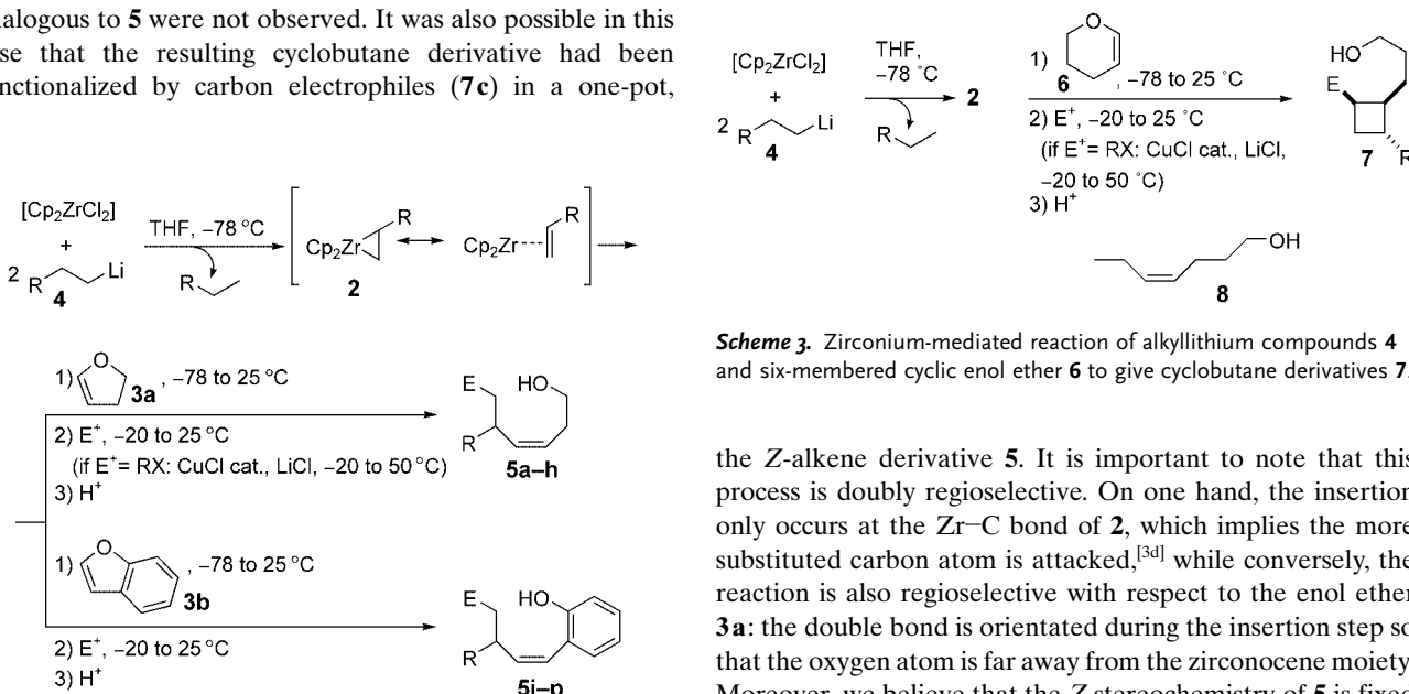
Scheme 2. Zirconium-mediated reaction of alkyl lithium compounds 4 and five-membered cyclic enol ethers 3 to give alkenol derivatives 5 .
