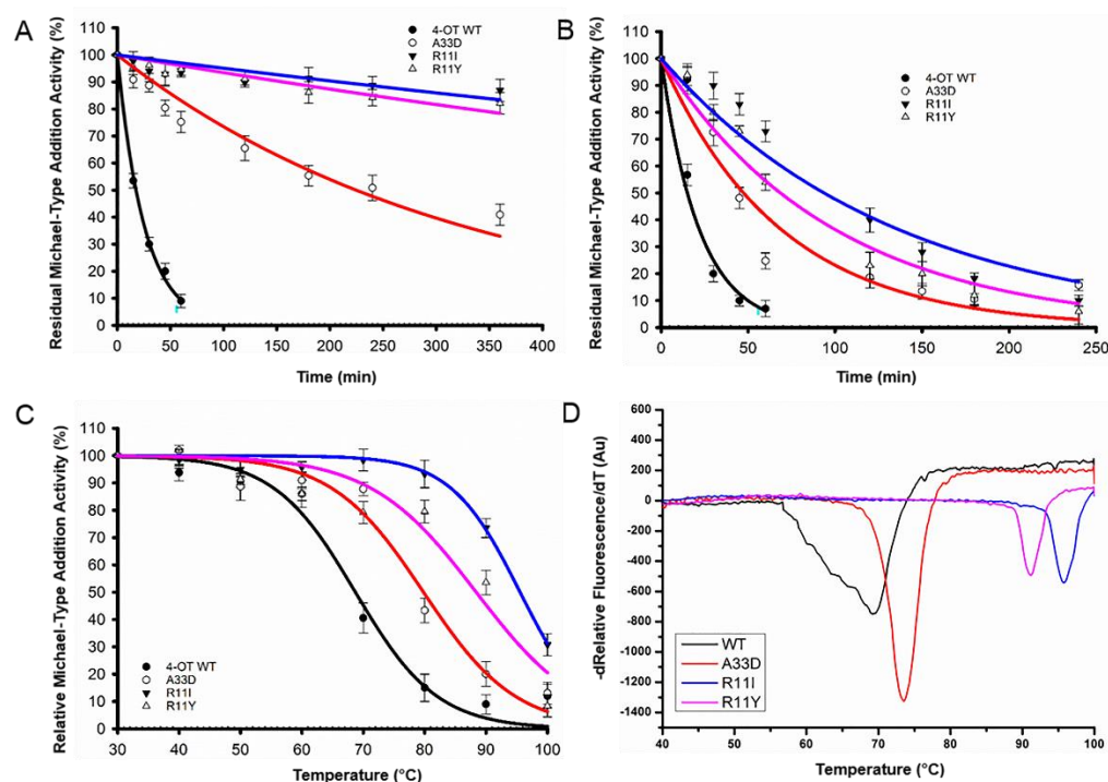
Figure 2. Thermostability assessment of wild-type 4-OT and the three single-mutant 4-OT variants. A) Activity decay at 80 °C. B) Activity decay at 100 °C. C) Determination of T_{50}^{120} values. D) The
