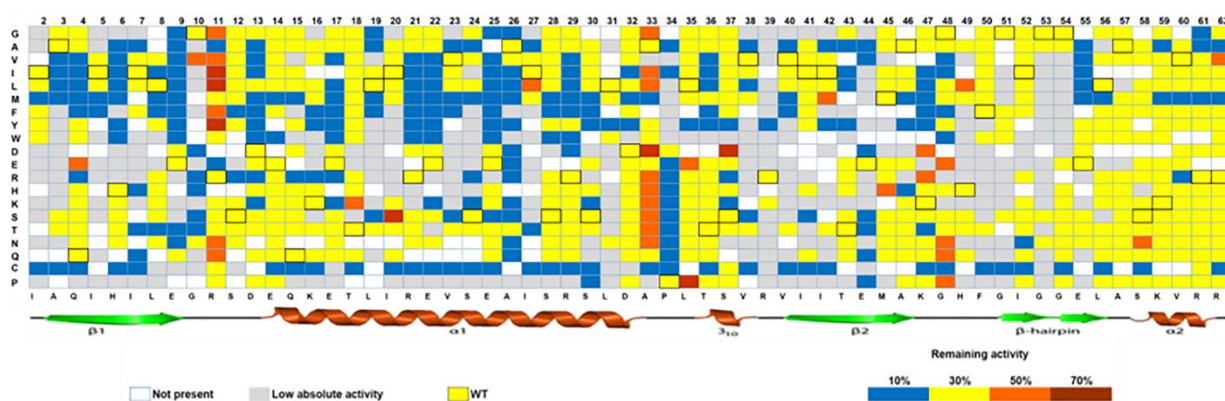
Figure 1. Thermostability mutability landscape of 4-OT. The horizontal axis of the data matrix represents the residue position of 4-OT, starting with Ile-2 and ending with Arg-62. The vertical axis represents all 20 canonical amino acids. For clarity, the wild-type amino acid at each position is indicated with a bold square. White squares indicate that this mutant is not present in the collection. The color of the other squares indicates the residual ‘Michaelase’ activity of 4-OT mutants after 1 h incubation at 80 °C compared to that after 1 h incubation at 25 °C. Grey boxes indicate that the ‘Michaelase’ activity was too low to determine the remaining activity. A “hotspot”
