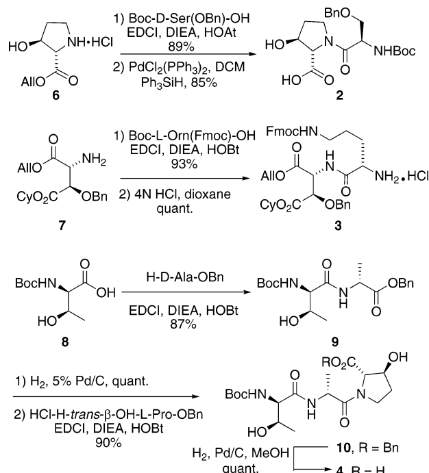
Scheme 2. Synthesis of Fragment 5
