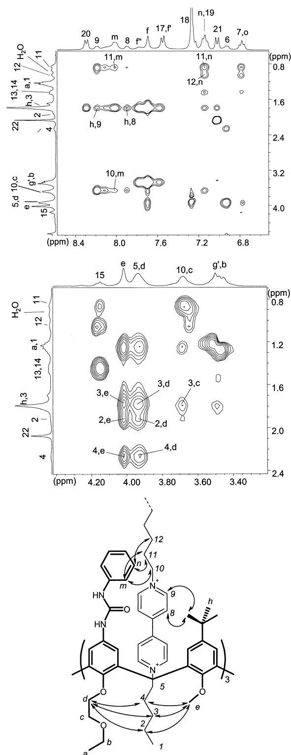
Figure 5. Selected expanded portions of ^1\text{H} 2D-ROESY NMR (300 MHz, spin-lock 200 ms) spectrum of pseudorotaxane 6b in \text{C}_6\text{D}_6 , showing the more representative axle–wheel intermolecular cross-peaks (for full 2D spectrum attribution see Supporting Information).
