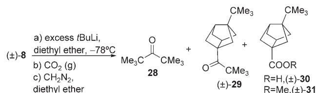
Finally, reaction of ( \pm )- 8 with excess t BuLi in anhydrous diethyl ether at -78^{\circ}\text{C} , followed by quenching of the reaction mixture with trimethylsilyl chloride, gave a very complex mixture from which no defined product could be isolated or identified. However, when the above reaction mixture was quenched by bubbling \text{CO}_2 (g), [13a] a very complex mixture of products was obtained as the neutral fraction, which by GC–MS analysis was shown to contain di- tert -butyl ketone ( 28 ) [17] (74.5% a.r.) and a compound whose mass spectrum is compatible for ketone ( \pm )- 29 (7.2% a.r.) as the main components (Scheme 8). Also, an acidic fraction was
