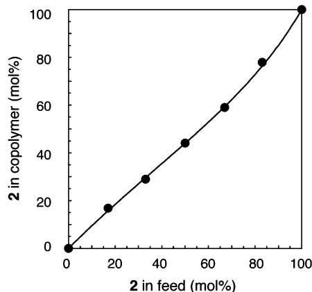
Figure 5. Relationship between the contents of 2 in copolymer and monomer feed in the copolymerization of 2 and 3 . Conditions: [M]_{0,\text{total}} = 0.11 M, [M]_{0,\text{total}}/[\text{catalyst}] = 50 in \text{DMF-}d_7 at 11–13% conversions, r_1 = 0.60 , r_2 = 1.02 . The line through the data points is theoretical, based on the r_1 and r_2 values.
