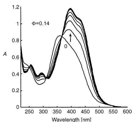
Figure 7. Irradiation at 313 nm of the cis -chalcone ( \text{Ct}^{2-} ) of 4'-hydroxy-6-nitroflavylium 1.25 \times 10^{-5} M at pH 12; from t = 0, 2.5, 5, 7.5, 10, 15, 20, 30, 40 min.
