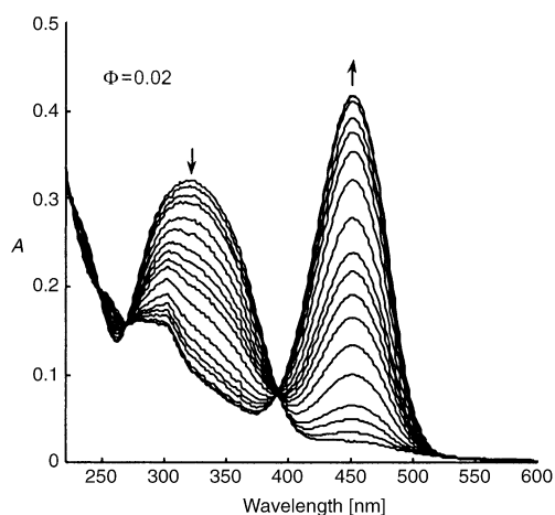
Figure 8. Spectral changes observed on irradiation at 313 nm of \text{Ct} 1.25 \times 10^{-5} M in [\text{HCl}] = 4 M; t = 0, 1, 3, 5, 10, 15, 20, 25, 30, 45, 60, 75, 90, 105, 135, 165, \text{ and } 195 min.
