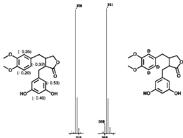
Figure 1 M + of unlabelled and deuterated 3,5-dihydroxy-3',4'-dimethoxylignano-9,9'-lactone. The isotopic purity of D 3 -product is over 95% according to MS. Electrostatic potential values (in parenthesis) were calculated to estimate the relative reactivities of the aromatic protons.
