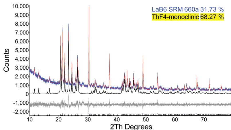
Figure 11. XRD powder pattern of the sample synthesized by heating (\text{NH}_4)_4\text{ThF}_8 at 800 °C for 60 min under \text{NH}_3(\text{g}) . The calculated pattern of \text{ThF}_4 is highlighted.
