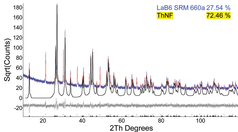
Figure 6. Observed (top continuous line) and calculated (highlighted continuous line for ThNF) patterns of ThNF synthesized by heating (\text{NH}_4)_4\text{ThF}_8 at 1100 °C for 15 min under \text{NH}_3 . Square root of counts was used as the scale of Y -axis for proper display of the calculated patterns.
