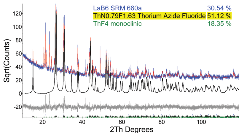
Figure 12. XRD powder refinement of the \text{ThF}_4 sample after the ammonolysis at 800 °C for 1 h. The calculated pattern of \text{ThN}_{0.79}\text{F}_{1.63} is highlighted. Square root of counts was used as the scale of Y-axis for proper display of the calculated patterns.
