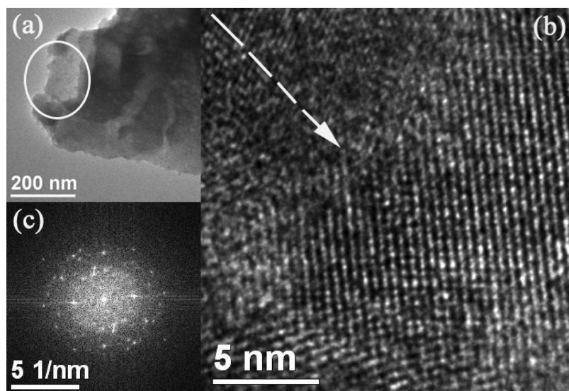
Figure 5. (a) TEM BF image of a ground (\text{NH}_4)_4\text{ThF}_8 particle. (b) The HRTEM image of the circled area of (a) and (c) the corresponding FFT.
