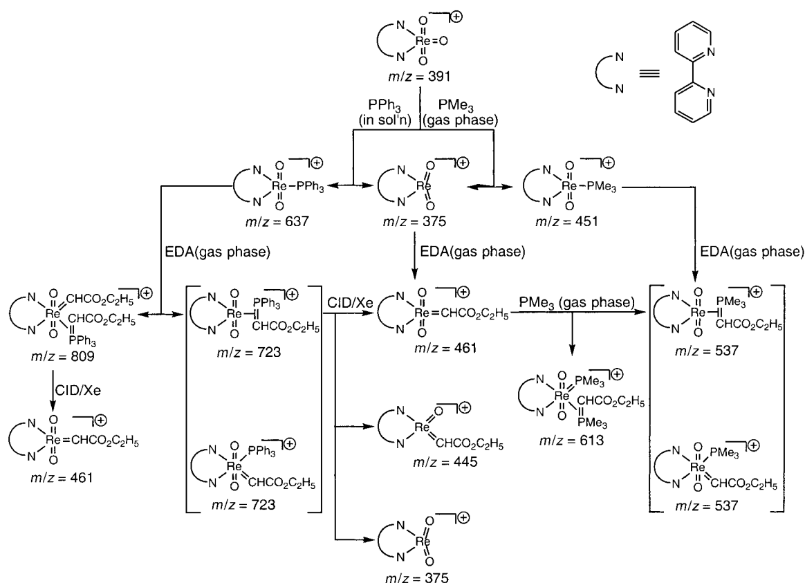
Scheme 1. Reactions of the [\text{ReO}_3(\text{bipy})]^+ ion ( m/z = 391 ) in solution and in the gas phase as evidenced by ESI mass spectrometry.
