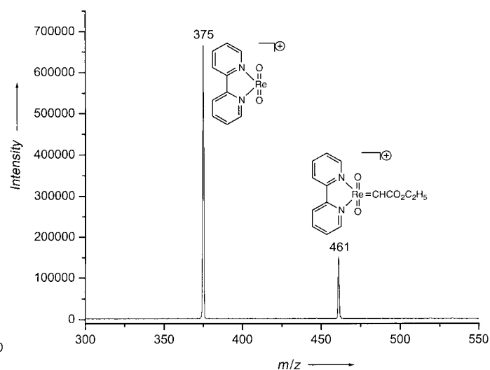
Figure 5. Daughter-ion spectrum produced by reaction of the mass-selected ion [\text{ReO}_2(\text{bipy})]^+ ( m/z = 375 ) with 0.38 mTorr ethyl diazoacetate in the octopole ion guide at low initial kinetic energy. The product ion at m/z = 461 can be assigned to [\text{ReO}_2(\text{bipy})(=\text{CHCO}_2\text{C}_2\text{H}_5)]^+ .
