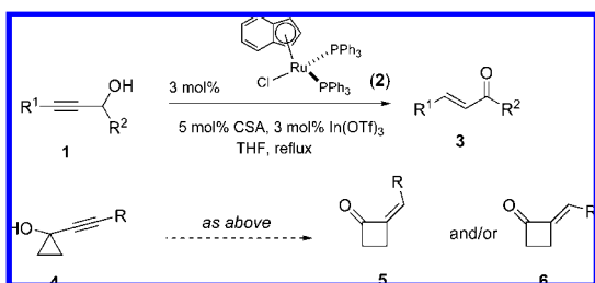
Scheme 1. Redox Isomerization and Proposal for a Ru-Catalyzed Ring Expansion of Alkynylcyclopropanols
