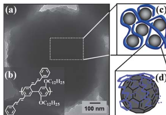
Fig. 1 TEM micrograph of 1 : 1 blend of C 12 -XXXX-C 60 hybrid nanocrystallites prepared in 0.1 mg mL -1 toluene solution (a) with inset showing the molecular structure of the polymer (b) and the proposed mechanism of formation (c–d).
