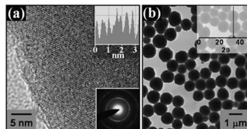
Fig. 2 High resolution TEM micrograph (a) of 1 : 1 blend of C 12 -XXXX-C 60 hybrid nanocrystallites prepared in 0.1 mg mL -1 toluene solution. The inter-lattice spacing measurement is in the upper inset and electron diffraction in the lower inset. The corresponding low magnification TEM (b) with an X-ray diffractogram in the inset shows monodispersed particles.
