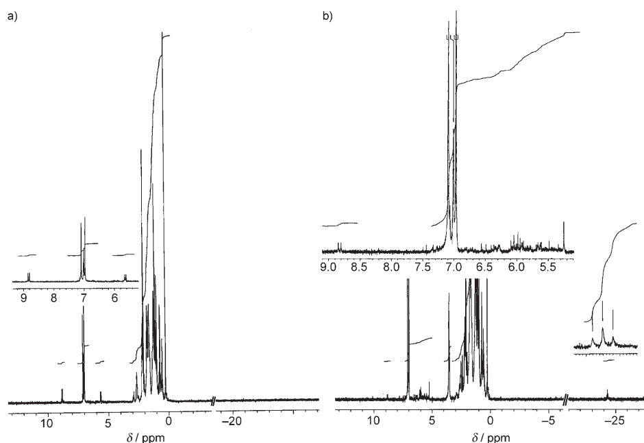
Figure 1. a) 1 H NMR spectrum of silylvinylene ruthenium complex generated in situ; b) 1 H NMR spectrum of the stoichiometric reaction of silylvinylene ruthenium complex with 2-vinyl-1,3-dioxaborolane, monitored after 24 h.
