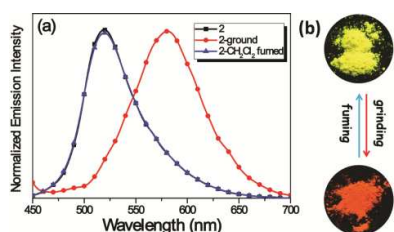
Figure 2. (a) Normalized luminescence spectra of solid compound 2 , after being ground and \text{CH}_2\text{Cl}_2 fumed, \lambda_{ex} , 414 nm. (b) Photographs of the ground powder of 2 and the \text{CH}_2\text{Cl}_2 -fumed ground powder under UV light (365 nm).
