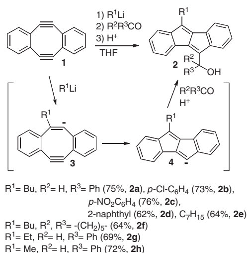
Scheme 1. Three component reaction through nucleophilic addition of R 1 Li to a triple bond of 1 followed by trans-annulation.
