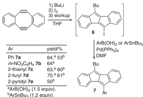
Scheme 3. Stepwise synthesis of 7 .
