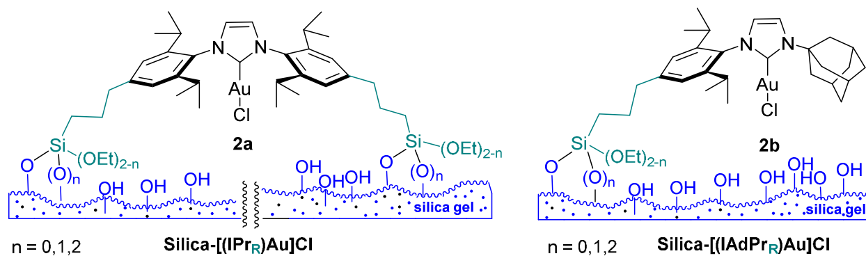
Chart 1. Silica immobilized catalysts 2a and 2b .
