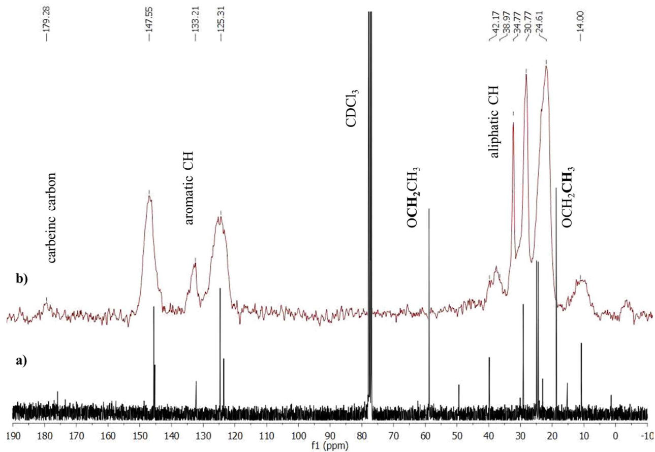
Figure 1. a) ^{13}\text{C} NMR spectrum of complex 9 in \text{CDCl}_3 solution; b) ^{13}\text{C} CP-MAS NMR spectrum of hybrid material Silica-[(IPr R )Au]Cl ( 2a ).
