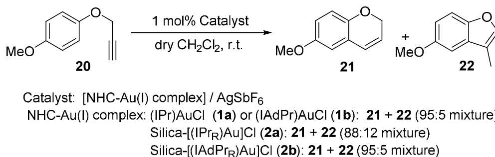
Scheme 3. Hydroarylation of arylalkyne 20 catalyzed by activated gold NHC complexes.
