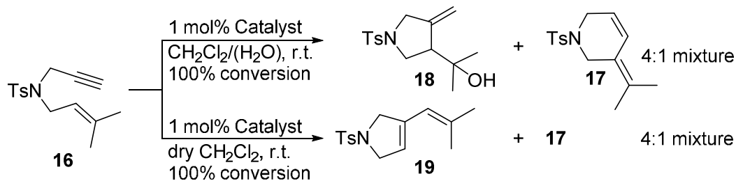
Scheme 2. Cycloisomerization of enyne 16 catalyzed by silica immobilized gold NHC complexes 2a and 2b .
