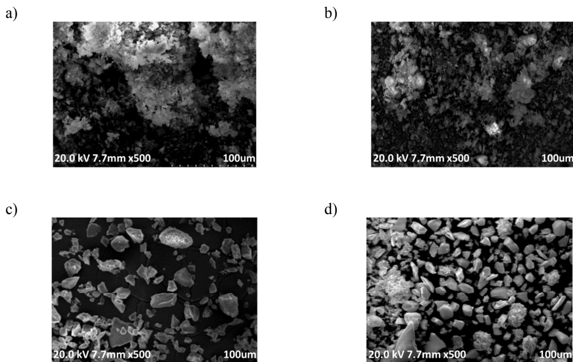
Figure 5. SEM images of a) hybrid silica material 2a after 12 cycles of hydration reaction; b) hybrid silica material 2b after 4 cycles of hydroarylation reaction; c) hybrid silica material 2b after 4 cycles of catalysis using an orbital shaker; d) hybrid silica material 2b after all the experiments carried out under continuous flow conditions.
