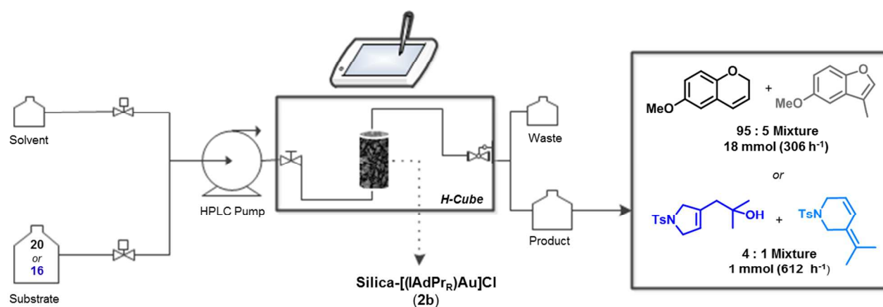
Figure 6. Hydroarylation and cycloisomerization carried out sequentially under continuous flow conditions catalyzed by 2b . Productivities in \text{mmol}_{\text{product}}.\text{mmol}_{\text{Au}}^{-1}.\text{h}^{-1} are shown in brackets.
