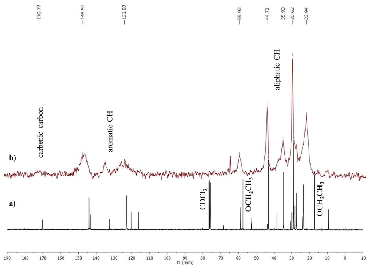
Figure 2. a) ^{13}\text{C} NMR spectrum of complex 11 in \text{CDCl}_3 solution; b) ^{13}\text{C} CP-MAS NMR spectrum of hybrid material Silica-[(IAdPr R )Au]Cl ( 2b ).
