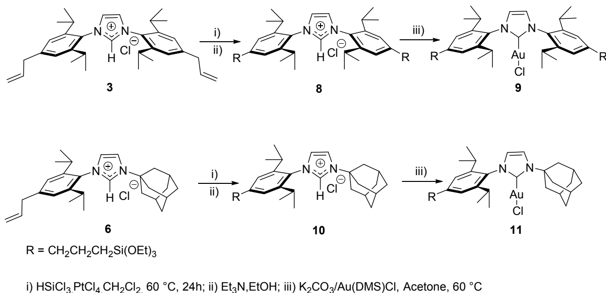
Scheme 1. Preparation of silylated gold complexes 9 and 11 .
