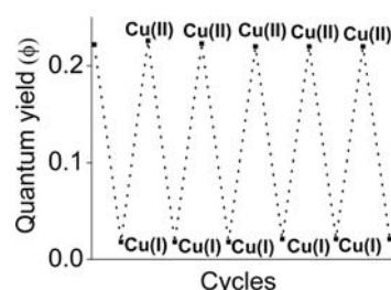
Fig. 3 Quantum yield plot of the L_1\text{-Cu(II)} complex after reduction by \text{NaBH(OAc)}_3 and subsequent aerial oxidation.
