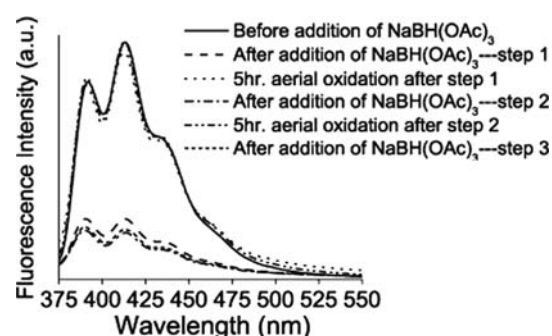
Fig. 2 Emission spectra of L_1\text{-Cu(II)} under different conditions.
