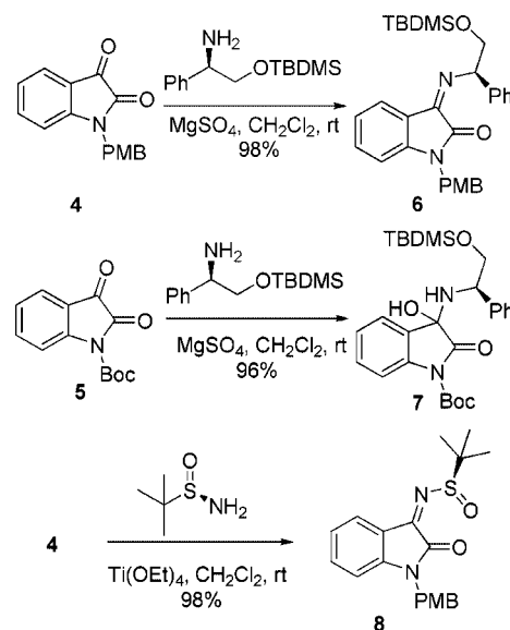
SCHEME 1. Synthesis of N-Protected Isatine-Based Imines 6 and 8 and of Aminal 7
