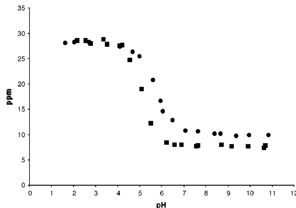
Figure 2. ^{11}\text{B} NMR chemical shifts of model compounds 6 (■) and 7 (●) with increasing pH (10% d_4 -methanol in water, 40 mM 6 and 7 , 40 mM NaCl). Referenced to \text{Et}_2\text{O} \cdot \text{BF}_3 in toluene as zero.
