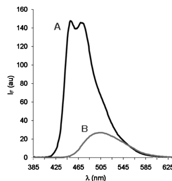
Figure 1. Fluorescence spectra of 3h (A) and Alq 3 (B) in the solid-state upon excitation at 380 nm.
