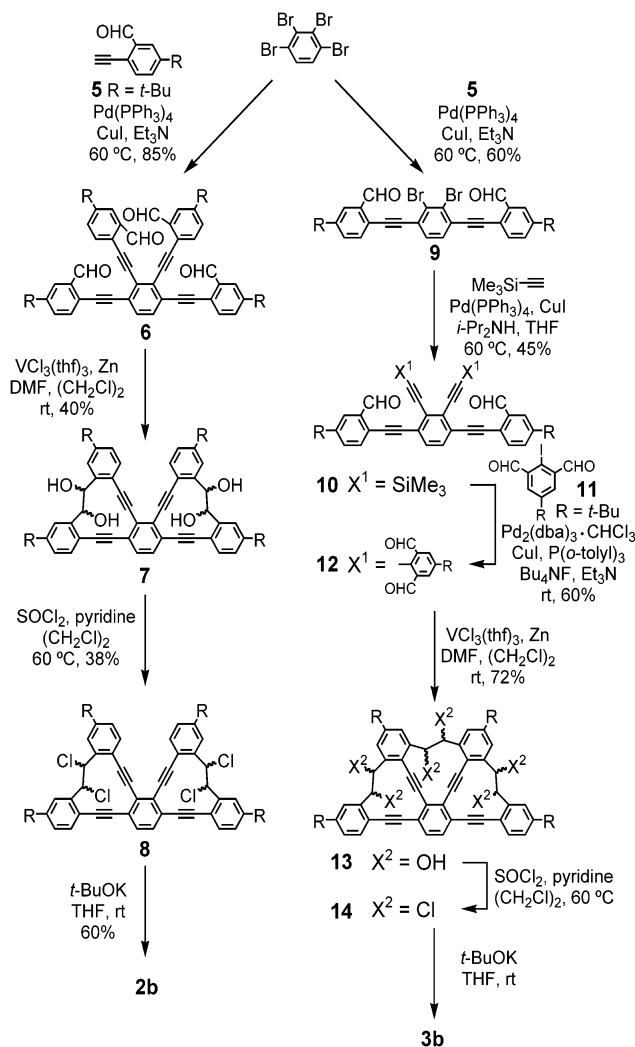
Scheme 1. Syntheses of bisDBA 2b and trisDBA 3b .
