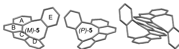
Figure 2. Single crystal X-ray diffraction analysis of constrained architecture 5 .
