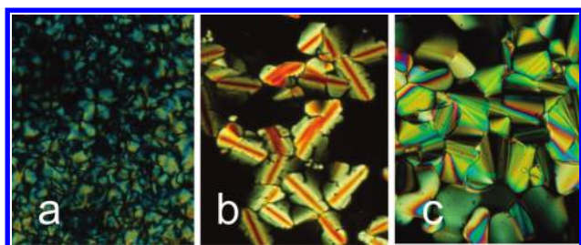
Figure 1. Polarized optical photomicrographs of mesophases for 5 at 92 °C (a), 6 at 25 °C (b), and 7 at 145 °C (c).
