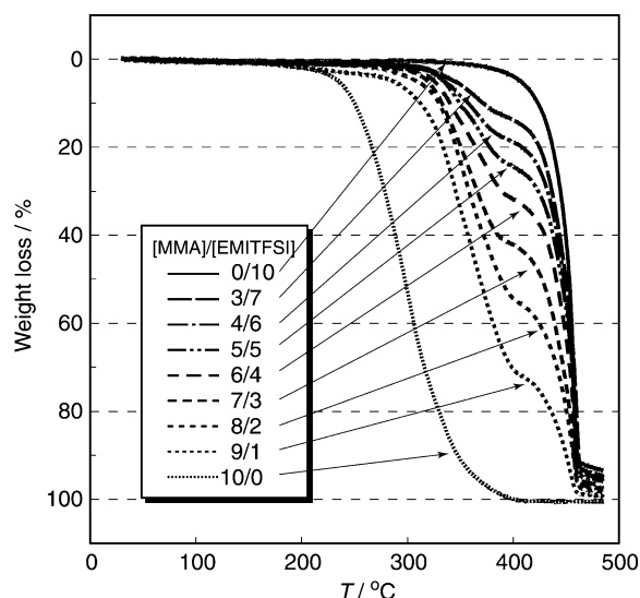
Figure 1. TG curves for MMA network polymers with different mole fractions of dissolved EMITFSI and EMITFSI bulk at a heating rate of 10 °C min -1 .
