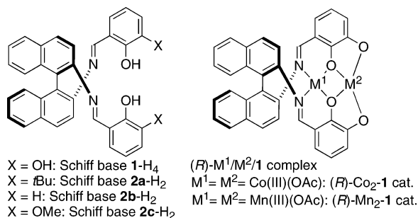
Figure 1. Structures of dinucleating Schiff base 1-H 4 , salen 2-H 2 , and bimetallic Schiff base 1 complexes.
