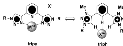
Scheme 1. Classical and Electronically Inverted Ligands
