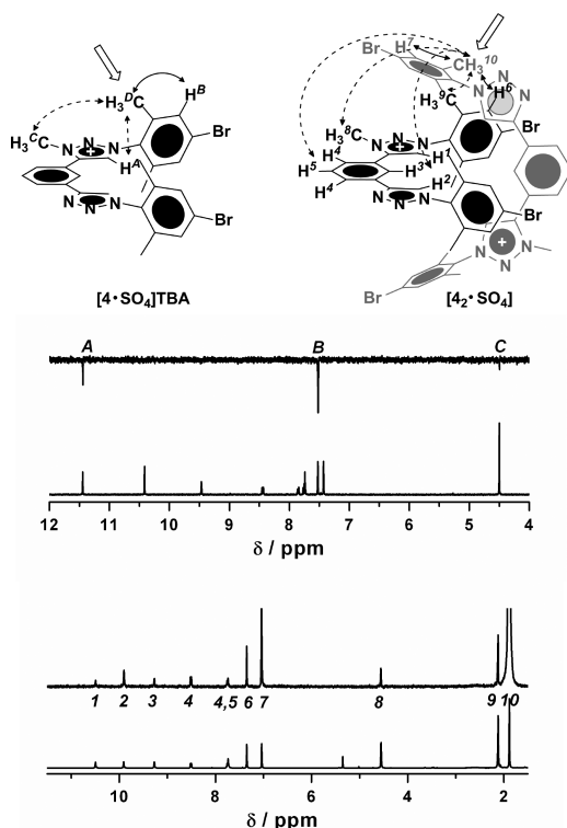
Figure 5. Selective NOESY spectra for [4 \cdot \text{SO}_4]\text{TBA} (top, acetonitrile- d_3 ) and [4_2 \cdot \text{SO}_4] (bottom, dichloromethane- d_2 ) (sulfate omitted; the excited protons are marked with a hollow arrow, and strong and medium NOESY contacts are indicated with solid and dashed arrows, respectively).
