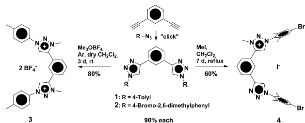
Scheme 2. Synthesis of the Anion Coordinating Ligands
