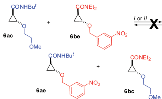
Scheme 2. Crossover Experiments Demonstrating Irreversible Addition of Alkoxide Species a
