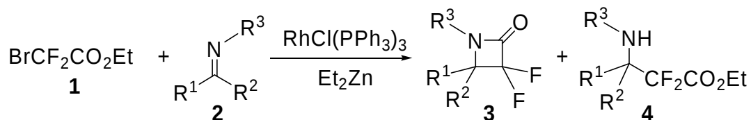
Scheme 1. Reaction of 1 with 2 in the presence of \text{RhCl(PPh}_3)_3
