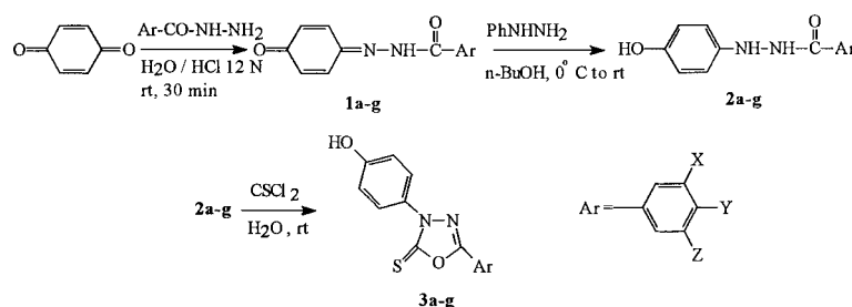
Fig. 1. Synthetic Route to 1,3,4-Oxadiazole-2(3H)-thione Derivatives 3a–g
