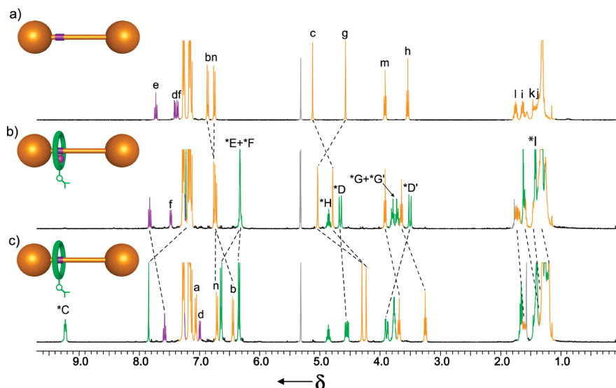
Figure 2. ^1\text{H} NMR spectra (400 MHz, \text{CD}_2\text{Cl}_2 , 298 K) of (a) thread L3 ; (b) palladium-complexed [2]rotaxane [ L4Pd ]; and (c) metal-free [2]rotaxane H 2 L4 . The lettering refers to the assignments in Scheme 1.
