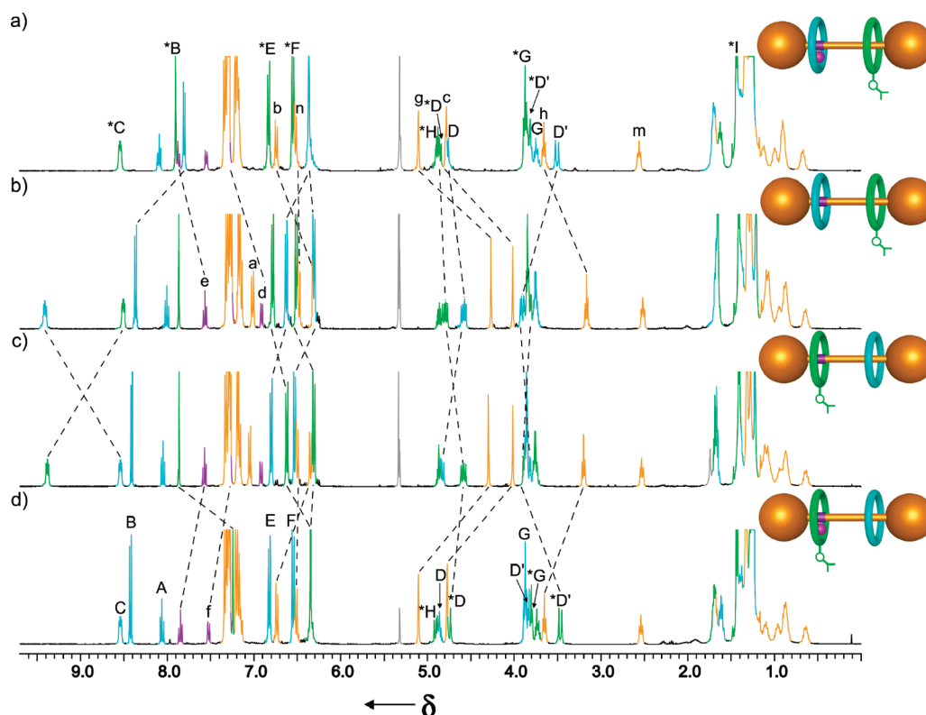
Figure 3. ^1\text{H} NMR Spectra (400 MHz, \text{CD}_2\text{Cl}_2 , 298 K) of (a) palladium-complexed [3]rotaxane [ L7Pd ]; (b) metal-free [3]rotaxane H 2 L7 ; (c) metal-free [3]rotaxane H 2 L6 ; (d) palladium-complexed [3]rotaxane [ L6Pd ]. The lettering refers to the assignments in Schemes 1 and 2.
