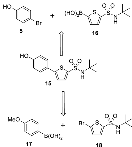
Scheme 4. Strategies for the synthesis of biaryl 15
