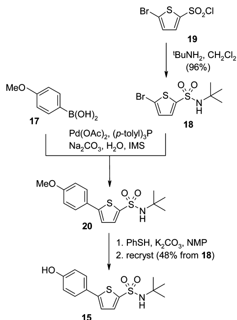
Scheme 5. First route for the synthesis of biaryl 15
